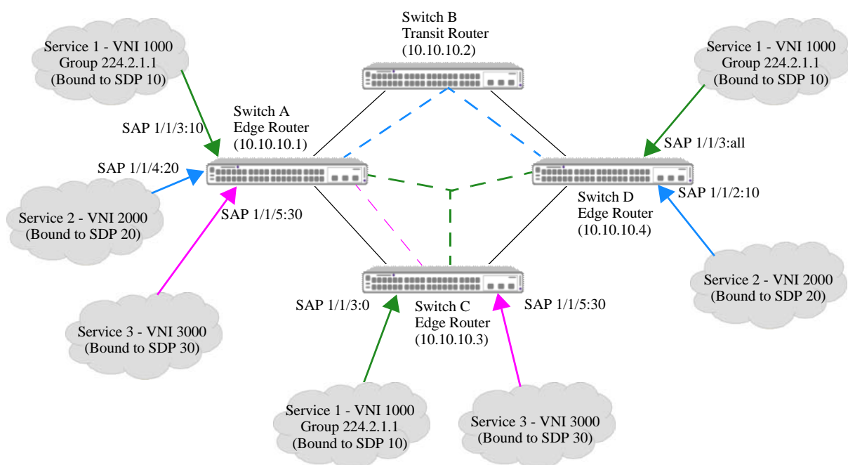
Figure 3: Sample VXLAN Configuration with Static Routes
